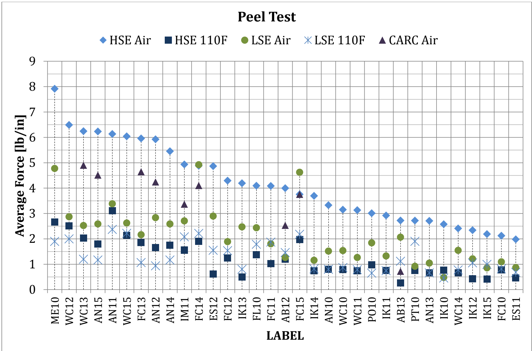
Figure 12. Average peel strength results by HSE substrate at room temperature.
