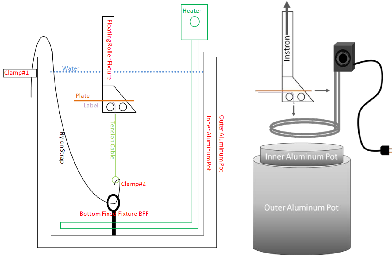
Figure 9. Sketch of heated peel setup. Left - inside water bath, Right - exterior sketch
