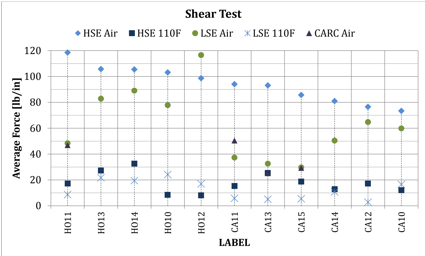
Figure 13. Average shear strength results by HSE substrate at room temperature.
