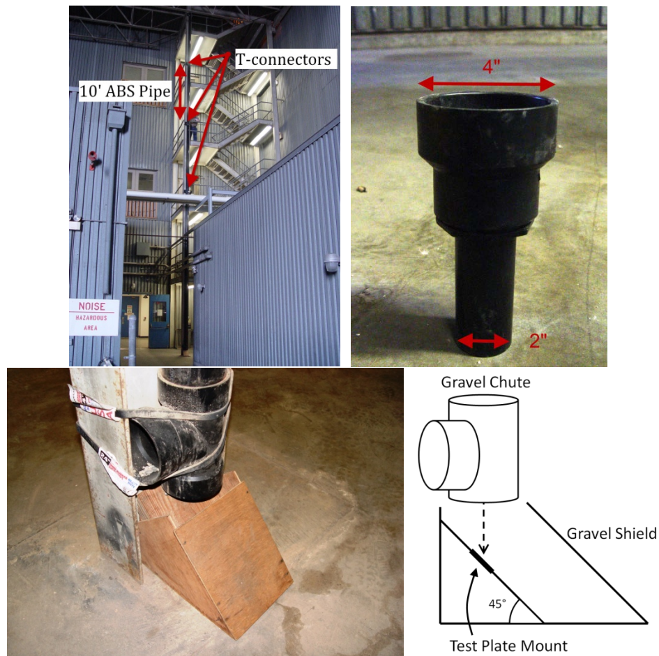
Figure 4. Views of the chipping tower, clockwise from top left: full tower, gravel collimator, side view diagram of gravel target, gravel target
