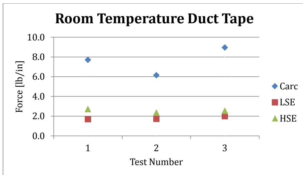
Figure 11. Room temperature adhesion strength of duct tape on multiple surfaces
