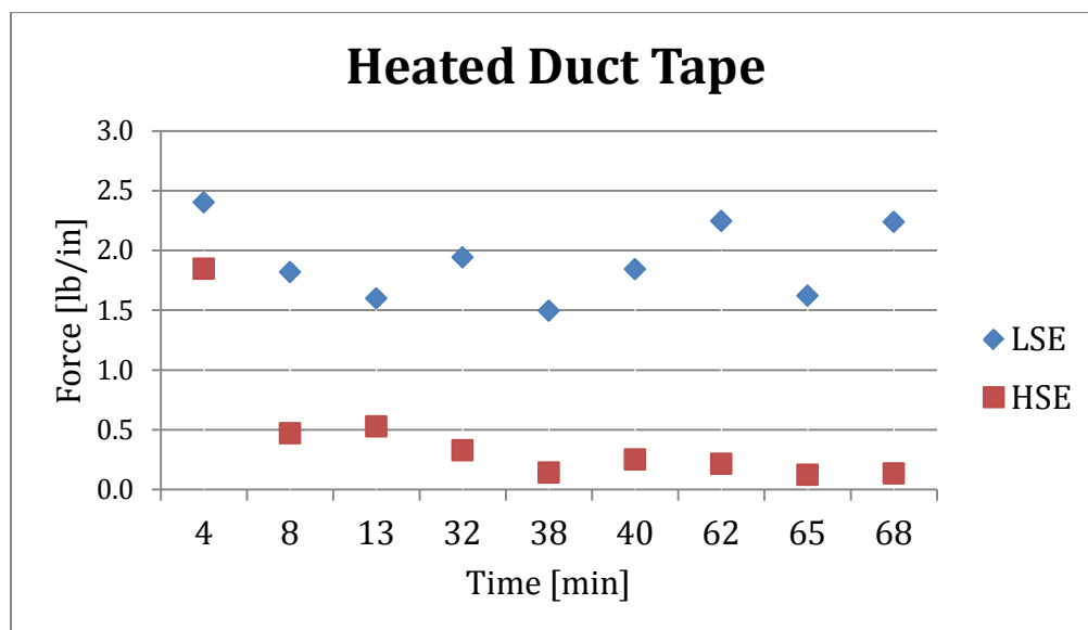
Figure 10. Duct tape immersion time vs. peel strength, one strip of tape tested at each time
