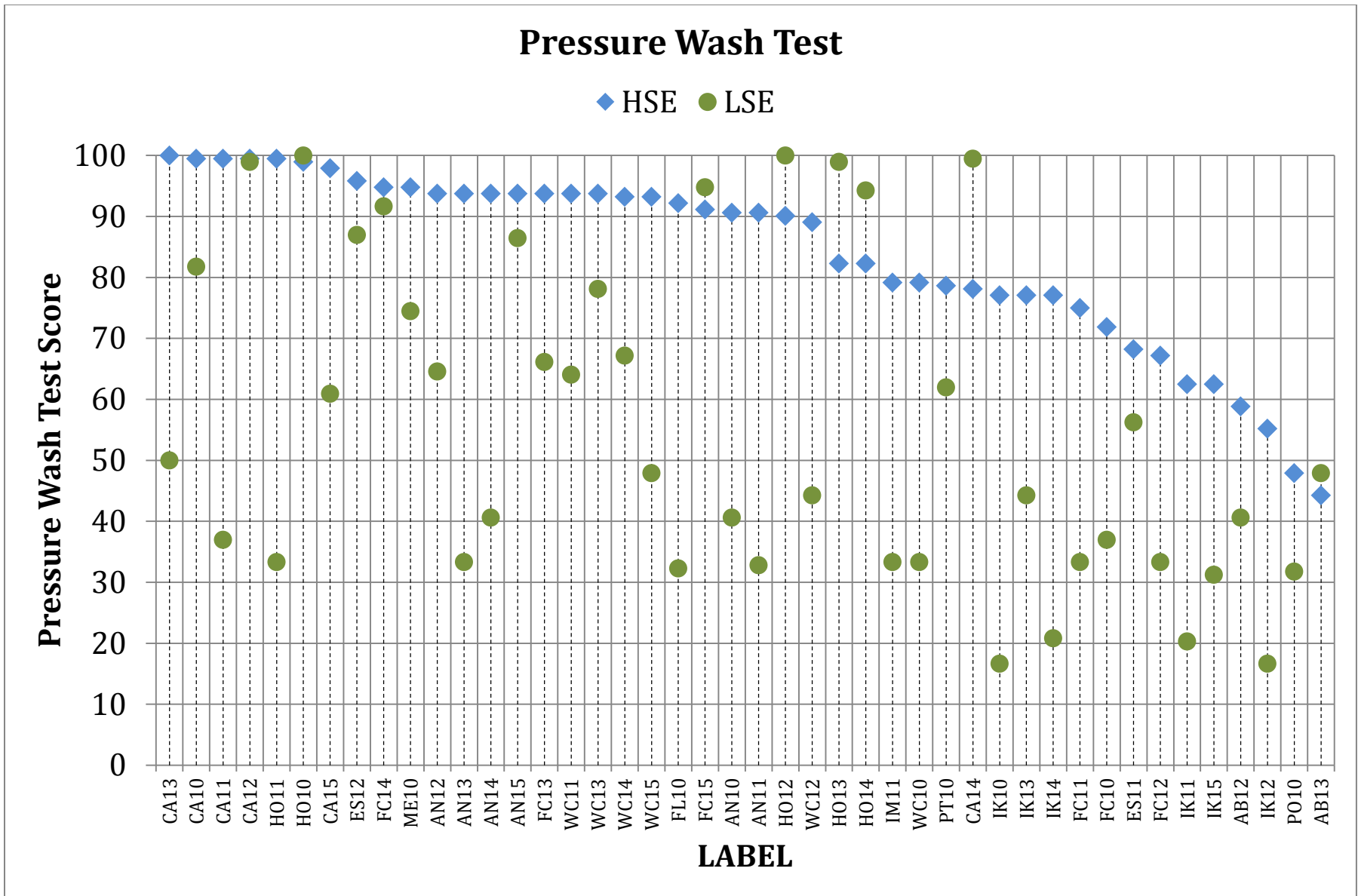
Figure 6. Plot of pressure wash scores by HSE substrate.
